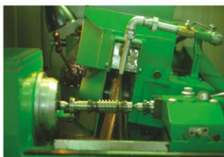
蜗杆磨床 Worm grinding machine
